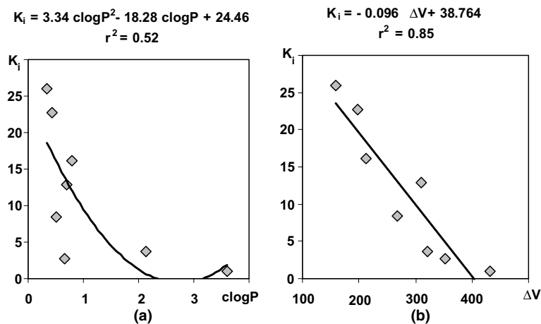
Figure 5. (a) Correlation between K_i -value at A_{2A} adenosine receptors and \text{clogP} . (b) Correlation between K_i -value at A_{2A} adenosine receptors and substituent volume.
