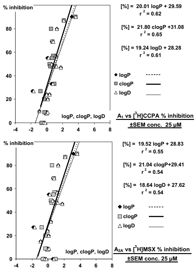
Figure 4. Relations between % inhibition of radioligand binding and lipophilicity descriptors.
