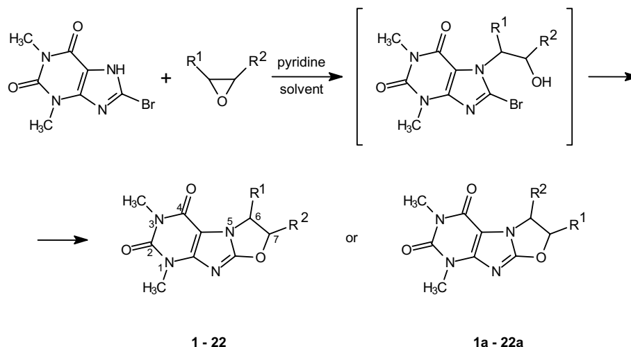
Figure 2. Synthesis of 7-mono or 6,7-disubstituted dihydrooxazolo[2,3- f ]purinediones.
